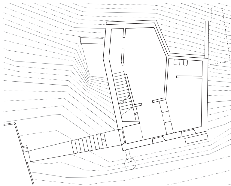
ERDGESCHOSS_GROUND FLOOR
